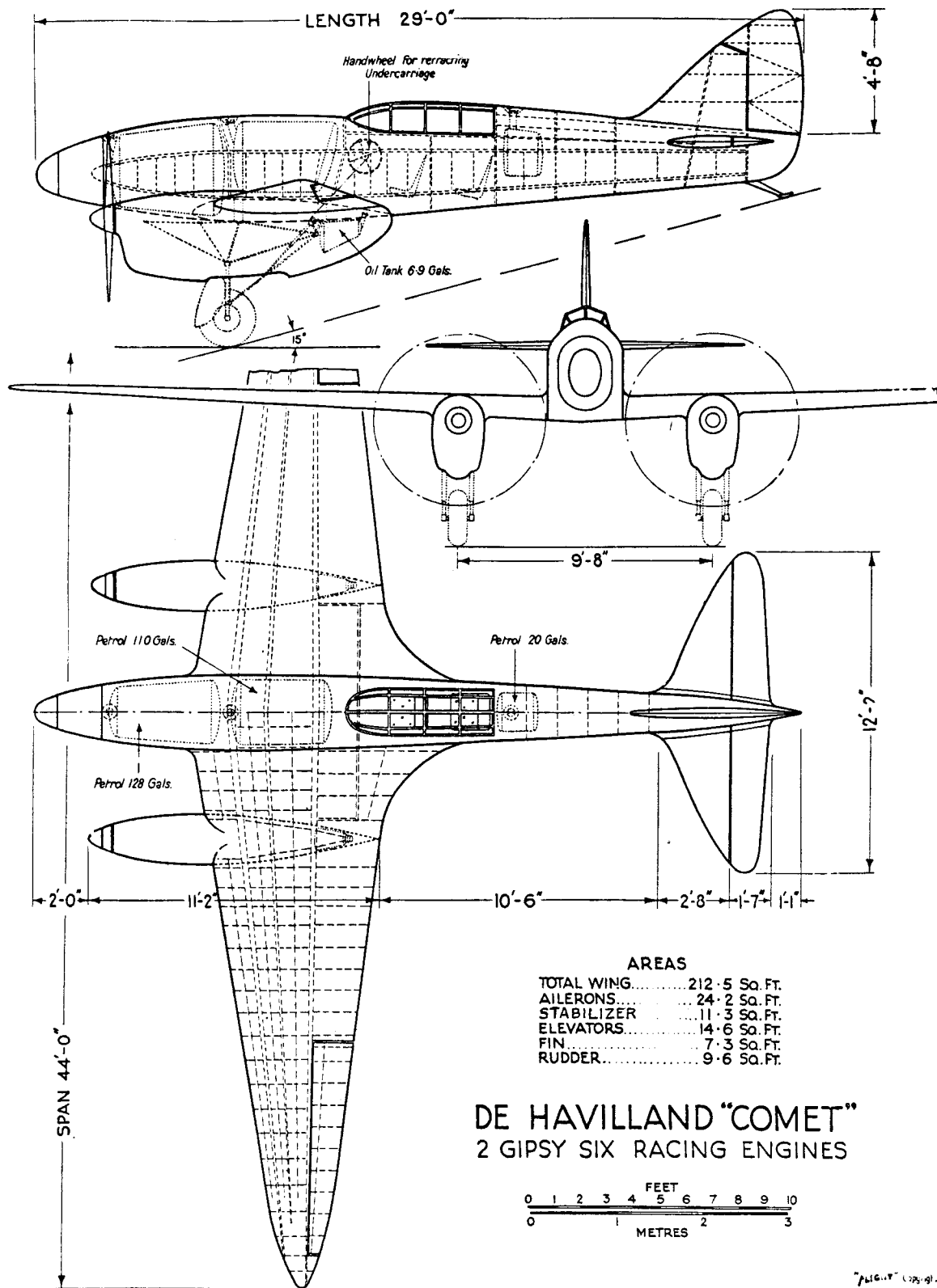
Figure 1.- General arrangement drawing of the DeHavilland Comet airplane.
