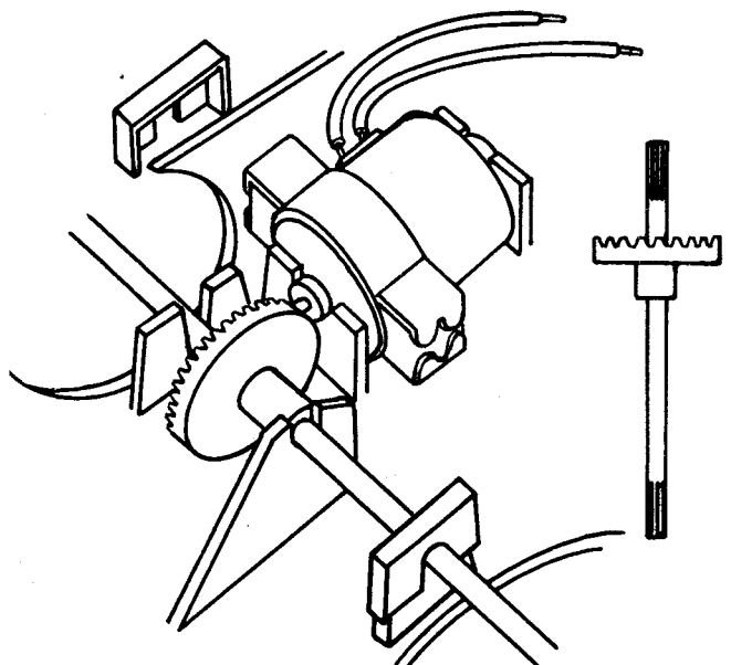
MOTOR MOUNTING DETAIL
