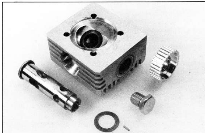
Webra's highly unusual cylinder head and rotary valve assembly. Rotary valve is of chromed brass. Toothed timing wheel is aluminum.
