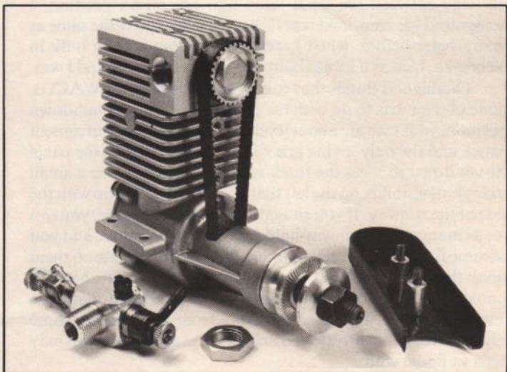
Simple toothed belt drive to rotary valve in head eliminates need for separate timing gears. Carburetor is Webra TN type.
