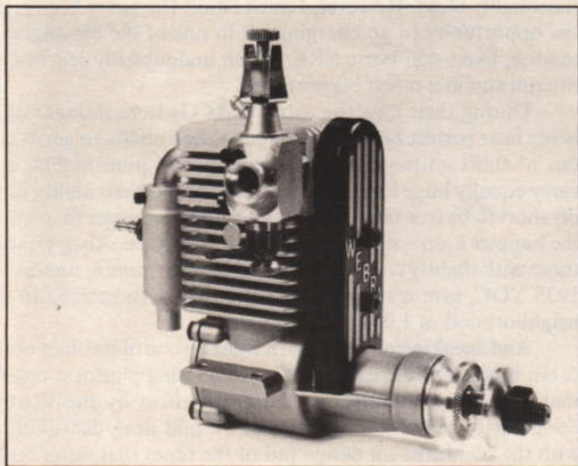
Webra's T4-40 is quite simple, no cams, rockers, pushrods, gears.
