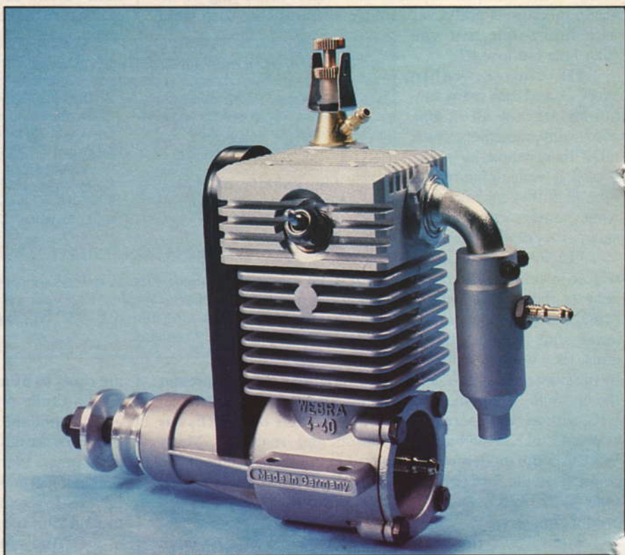
Engine comes complete with muffler, which also provides pressure take-off for fuel tank. Fitting in backplate is crankcase breather.
