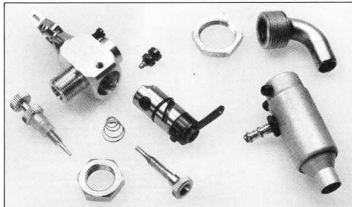
Carburetor parts, left, showing two needles and O-ringed throttle barrel. Exhaust elbow and muffler assembly on right.
